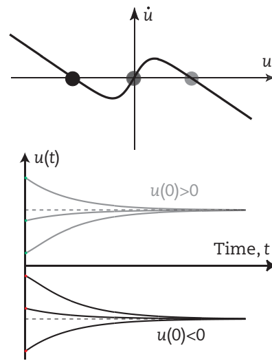
FIGURE 1.16: Top: Dynamics of a single activation variable with self-excitation, \tau \dot{u} = -u + h + s(t) + c \cdot g(t) , in the presence of external input, s(t) = \text{constant} of intermediate strength. The dynamics has an attractor at a negative activation level (circle filled in solid black) and another one at a positive activation level (circle filled in light gray), separated by a repeller at zero activation level (circled filled in dark gray). Bottom: Simulated activation trajectories converge to the positive attractor (dashed line in light gray) when started at positive initial activation levels (light gray curves) and to the negative attractor (dashed line in solid black) when started at negative initial activation levels (solid black curves). This shows that the dynamics is bistable.
