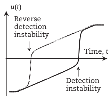
FIGURE 1.17: The dynamics of a single activation variable with self-excitation, \tau \dot{u} = -u + h + s(t) + c \cdot g(u) , is simulated when external input, s(t) , is first increased, then decreased, in both cases linearly over time. The resulting activation level is shown as a solid line for increasing input and as a dashed line for decreasing input (plotted against a reversed time axis). The dependence of the realized activation level on the direction of change of input is a signature of hysteresis.
